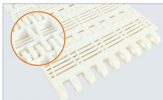
Pitch = 50.8mm Open area: 23% NET Code: N5080-UOPB4V-FG23
