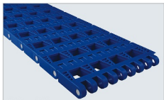
Pitch = 50.8mm Open area: 36% NET Code: N5080-UOPB4V-FG36
