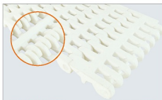
Pitch = 50.8mm Open area: 22% NET Code: N5080-UMPB-FG22
