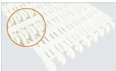
Pitch = 50.8mm Open area: 20% NET Code: N5080-UMPB-FG20
