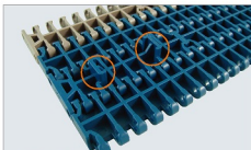
Pitch = 25.4mm NET Code: N2540-R1000-FT(DP)
