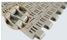
Pitch = 19.05mm Open area: 16% NET Code: N1905-R5936-FG
