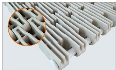
Pitch = 50mm Open area: 36% NET Code: N5000-ULSNB-RR
