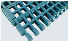
Pitch = 25.4mm Open area: 40% NET Code: N2540-R1000-FG
