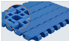
Pitch = 25mm NET Code: N2500-E502A-FT
