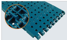
Pitch = 25.4mm Open area: 10% NET Code: N2540-R1000-VT(DP)
