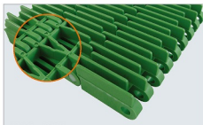
Pitch = 50.8mm Open area: 23% NET Code: N5080-UOPB4V-RR
