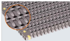
Pitch = 19.05mm Open area: 20% NET Code: N1905-R8506-FG
